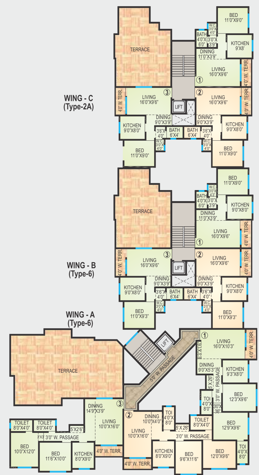
AGARWAL HEIGHTS (SEVENTH FLOOR PLAN)
