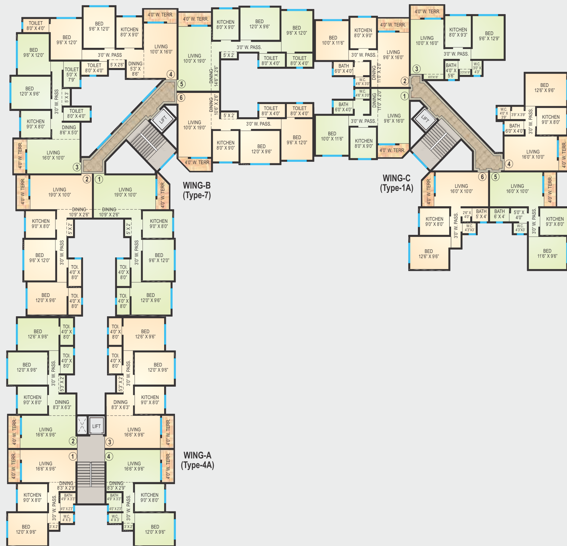
AGARWAL PARADISE (THIRD, FIFTH & SEVENTH FLOOR PLAN)
